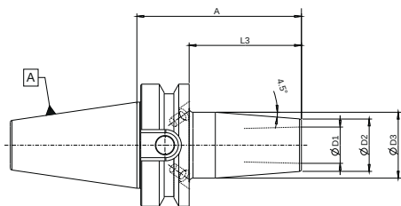
TMG14...JD40_BT40, TMG14...FBT40
