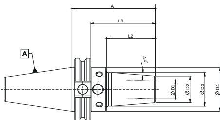
TMG14...CAT40
